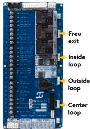
Smart Touch Controller Board
