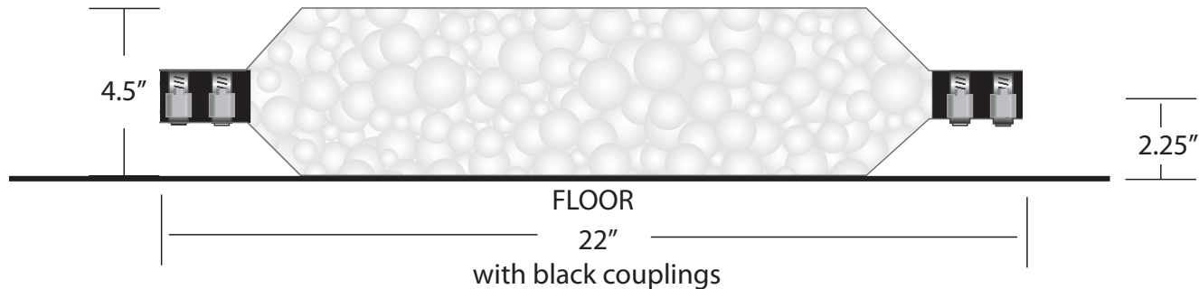
SIDE VIEW
