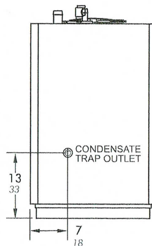
BACK VIEW
