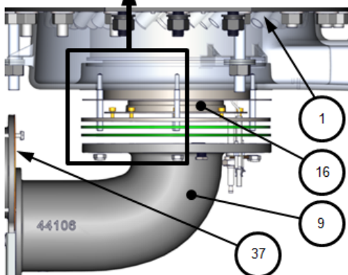
RIGHT-SIDE VIEW – EXPLODED
